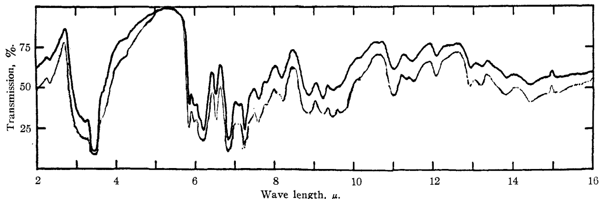
Fig. 2.—Infrared absorption spectra (mineral oil mull): —, natural crotonoside; — —, 9-β-D-ribofuranosylisoguanine.
